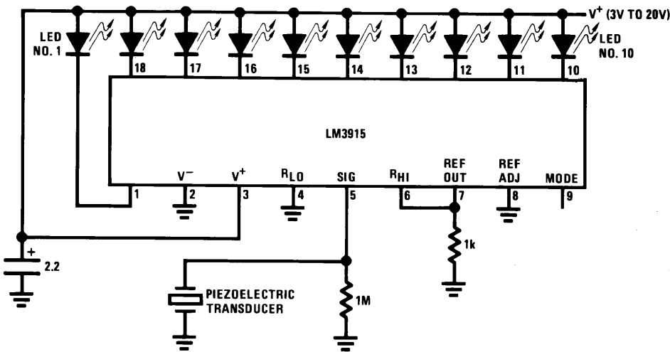
Figure 29. Vibration Meter
